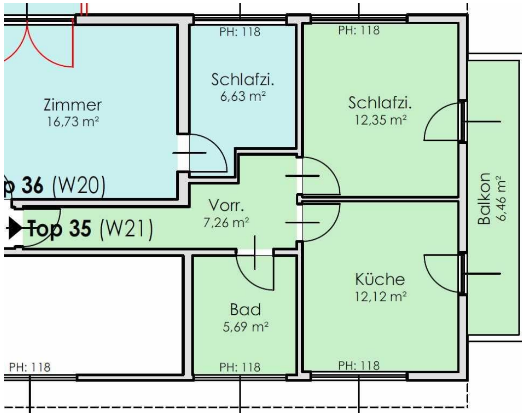
Grundriss / floor plan
